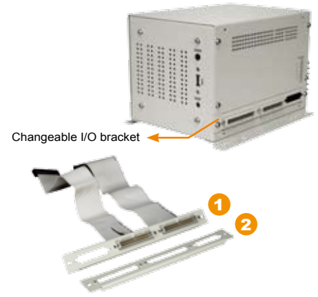
1. I/O bracket with 40-pin and 34-pin ribbon cables 2. I/O cable without cables
